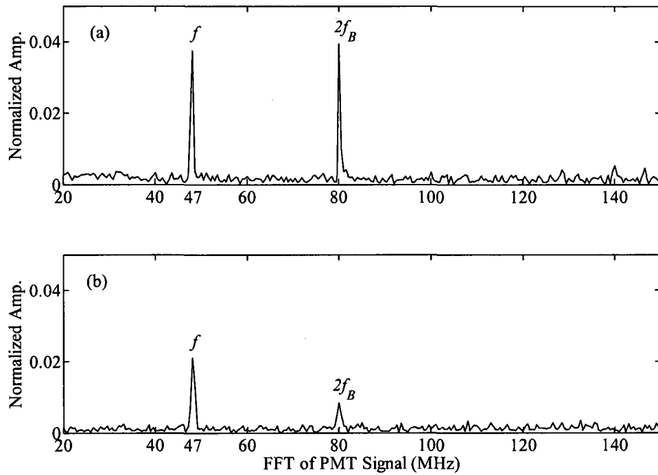
Figure 2.12: Temporal intensity spectra of the 488 nm LDV signal beam with 2L/\lambda \sim 15 (a) and 2L/\lambda \sim 30 (b). The Bragg angle was optimized for 488 nm. The amplitude of the Bragg Cell induced intensity fluctuation is comparable to the LDV burst signal, and is reduced by laser beam expansion. No frequency mixing peaks are detected.
