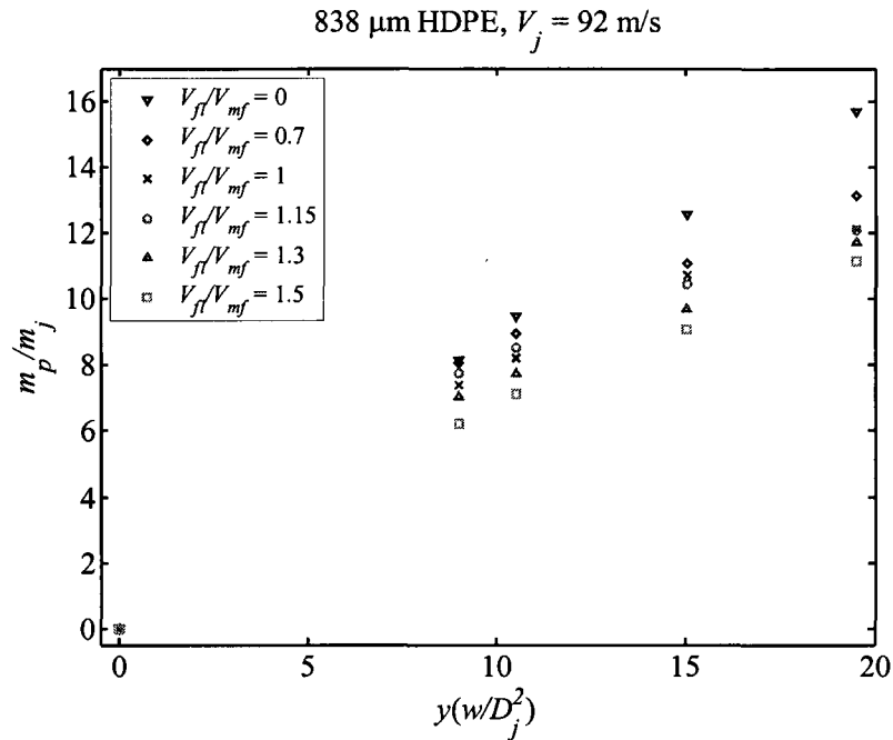
Figure 6.10: Mass flow rates for the particulate phase with varying fluidization velocity. As the fluidization rate increases, the particulate phase mass flow decreases due to competition with the increased interstitial gas entrainment.
