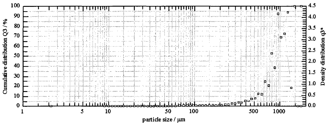
Figure 5.2: Particle size distribution for the HDPE microspheres. Data acquired via laser diffraction techniques. SMD = 838 \mu\text{m} , VMD = 910 \mu\text{m} .
