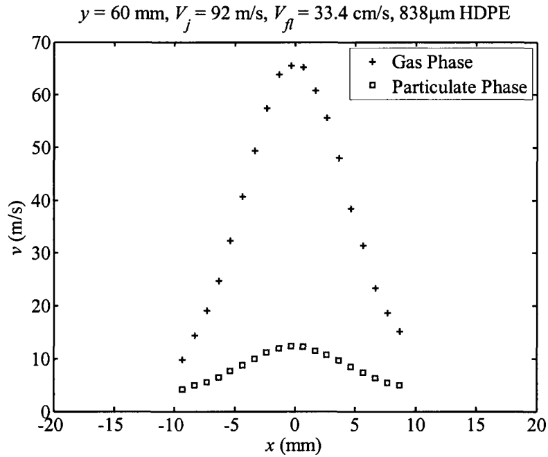
Figure 3.13: Gas and particulate phase velocity profiles at y = 60 \text{ mm} in the vertical jet.
