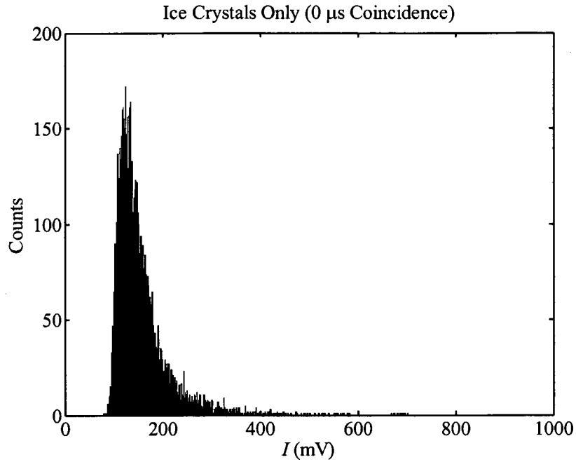
Figure 3.7: Histogram of ice crystal Doppler burst intensity.
