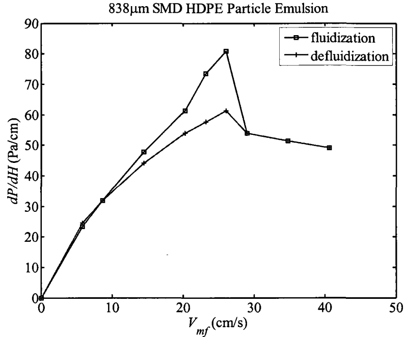
Figure 5.3: Fluidization and defluidization curves for the 838 \mu\text{m} HDPE micropellets. The minimum fluidization velocity was experimentally determined to be 29 cm/s.
