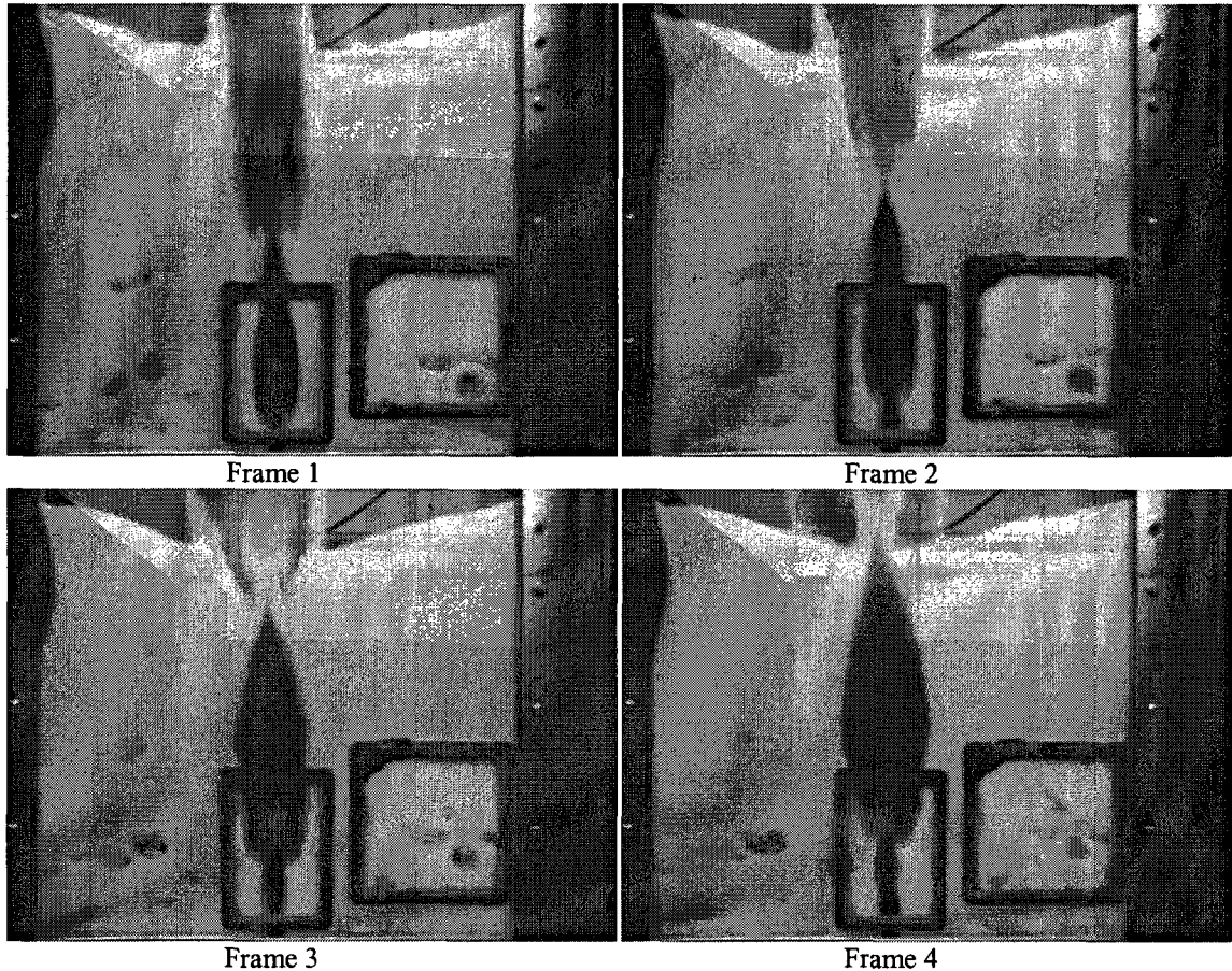
Figure 5.1: Vertical gas jet in the 2D bubbling fluidized bed. The jet inlet velocity is 92 m/s and inlet momentum is 0.735 \text{ kg.m/s}^2 . The emulsion of 838 \mu\text{m} HDPE particles was fluidized at a velocity of 33.4 cm/s, about 15% beyond minimum fluidization. Sequential images captured at 30 FPS.
