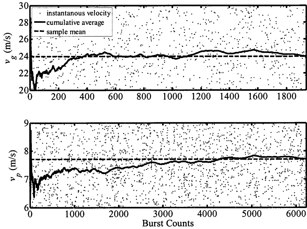
Figure 5.37: LDV gas and particulate phase velocity measurements at y = 130 \text{ mm} , x = 10 \text{ mm} . 1,938 bursts were recorded for the gas phase and 6,231 bursts for the particulate phase over the recording period of 120 seconds.
