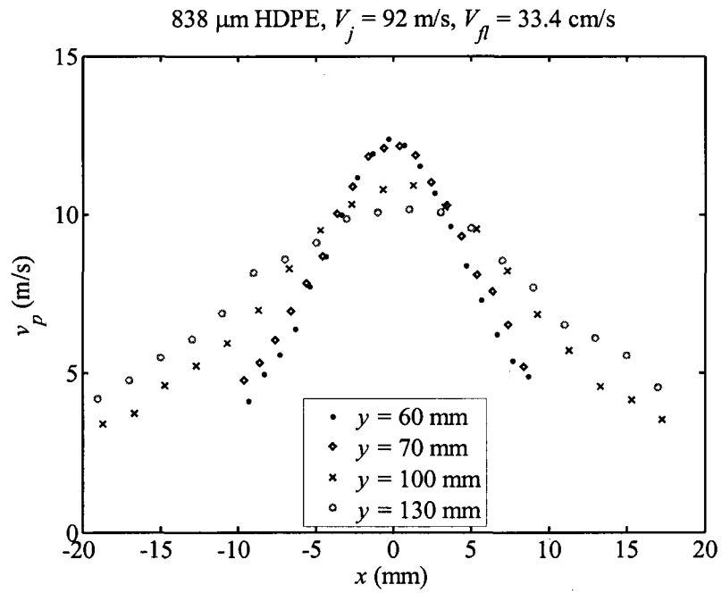
Figure 5.5: Particulate phase velocity profiles.
