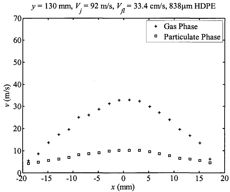
Figure 3.16: Gas and particulate phase velocity profiles at y = 130 \text{ mm} in the vertical jet.
