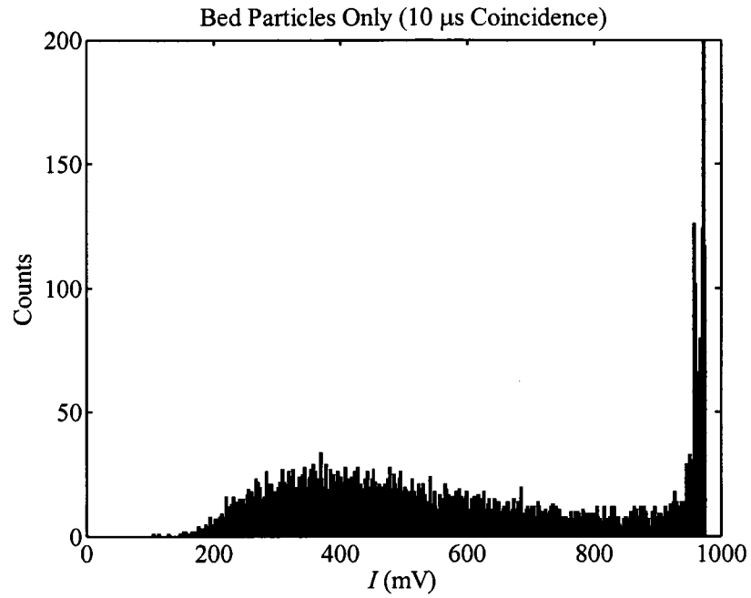
Figure 3.5: Histogram of bed particle Doppler burst intensity.
