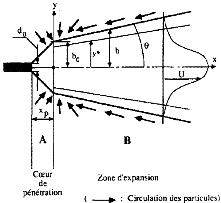
Figure 1.7: Schematic of a horizontal gas jet in a bubbling fluidized bed (Xuereb et al. , 1992). Particles propagate along the plume boundary in the emulsion towards the jet nozzle where they are entrained. The jet experiences an initial penetration zone following by a region of linear expansion where the average velocity profile is assumed to be Gaussian and self-similar in shape.
