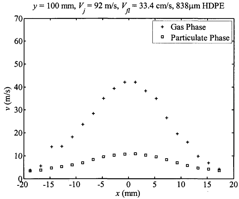
Figure 3.15: Gas and particulate phase velocity profiles at y = 100 \text{ mm} in the vertical jet.
