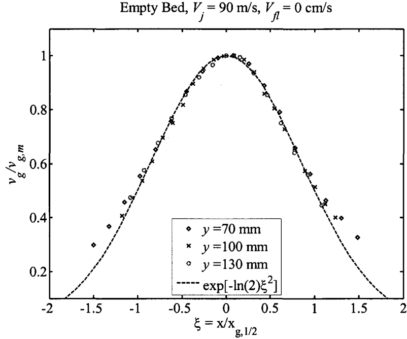
Figure 4.14: Normalized gas phase velocity profiles scaled with respect to the half-velocity points and compared to the Gaussian profile.
