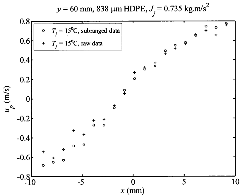
Figure 5.38: Particulate phase lateral velocity profiles at y = 60 \text{ mm} .
