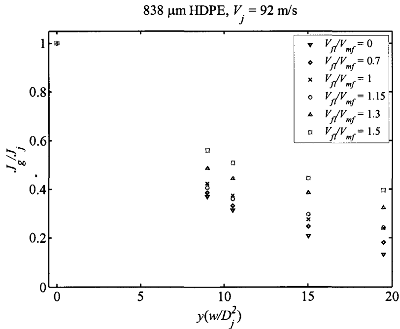
Figure 6.11: Momentum rates for the gas phase with varying fluidization velocity. As the fluidization rate increases, the gas phase momentum increases due to increased interstitial gas entrainment.
